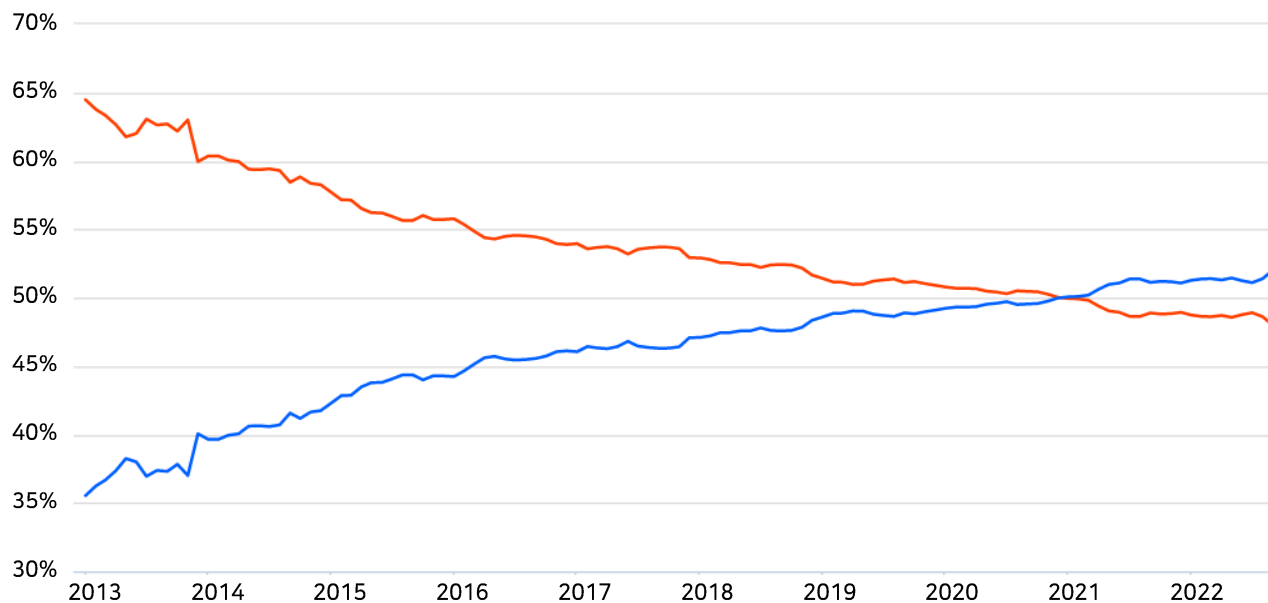
Popularity trend
